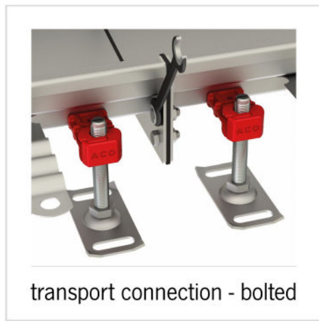
transport connection - bolted
